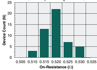
Typical On-Resistance Distribution (N=50, I F =1mA, I L =400mA)
