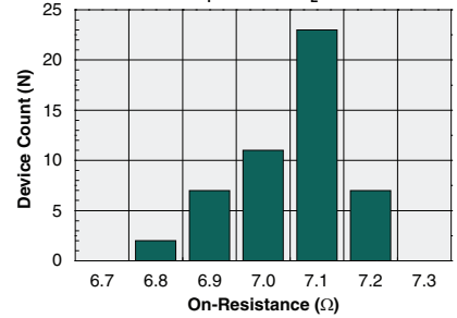
Typical On-Resistance Distribution (N=50, I_F=0.5\text{mA} , I_L=75\text{mA} )
