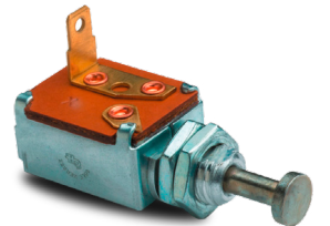
91812 12V 5A Normally Closed Self Grounded Door Switch
