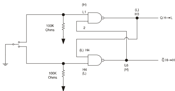
Figure 5. Circuit anti-rebond
