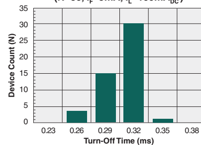
Typical Turn-Off Time (N=50, I_F=5\text{mA} , I_L=100\text{mA}_{DC} )
