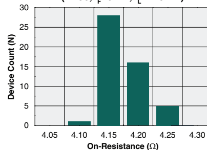
DC-Only On-Resistance Distribution (N=50, I_F=5\text{mA} , I_L=220\text{mA} )
