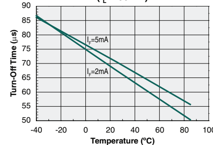
Form-A Typical Turn-Off Time vs. Temperature ( I_L=100\text{mA} )
