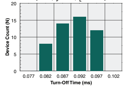
Form-A Typical Turn-Off Time (N=50, I_F=5\text{mA} , I_L=100\text{mA} )
