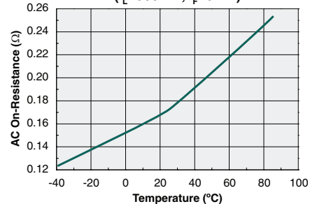
Form-A Typical On-Resistance (AC) vs. Temperature ( I_L=500\text{mA} , I_F=5\text{mA} )
