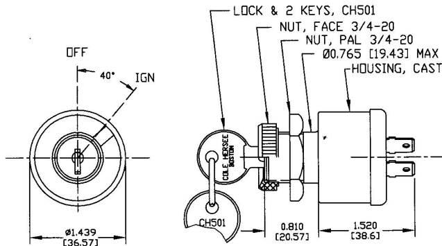
FRONT VIEW LESS KEYS, FACENUT & PALNUT
