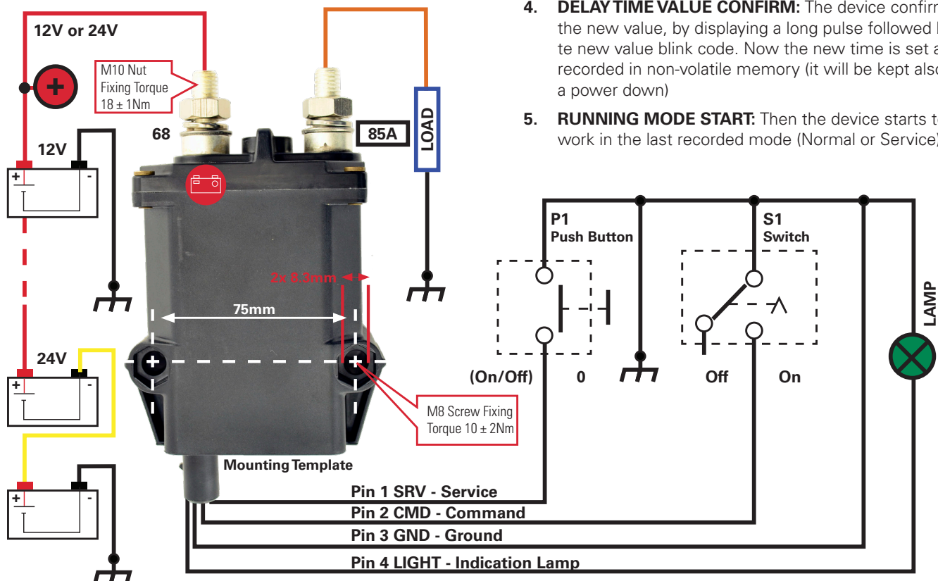
Figure 1 - Installation Diagram TGC/RME-M2 • 12/24V + 100°C
