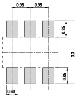
Recommended soldering pad layout (unit :mm)
