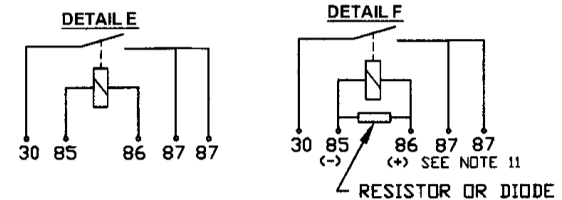
FORM 2 (SPST) W/ SUPPRESSION
