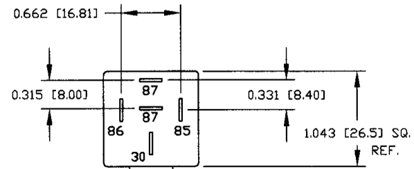
FORM 2 TERMINALS BOTTOM VIEW
