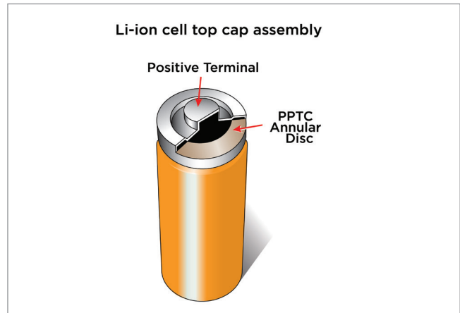
Figure 8. A PolySwitch disc device's placement on an 18650 battery cell.
