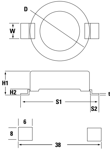
Soldering Pad Layout
