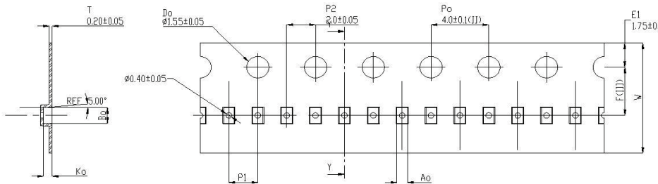
Component Orientation in Tape
