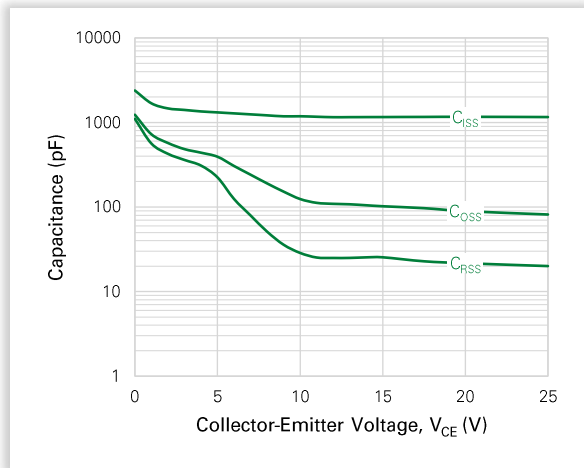
Figure 10. Capacitance Variance
