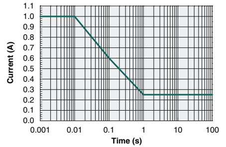
Maximum Non-Repetitive Surge Current ( T_A=25^\circ\text{C} )
