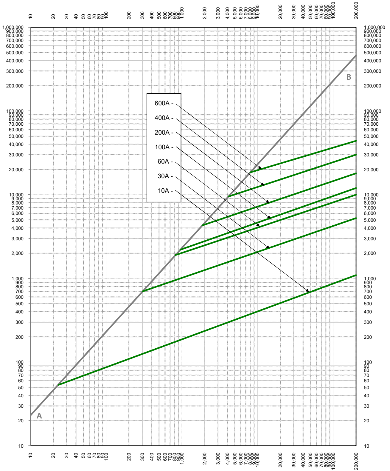
AVAILABLE FAULT CURRENT SYMMETRICAL R.M.S. AMPERES
