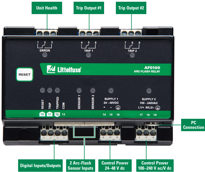
AF0100 Arc-Flash Relay
