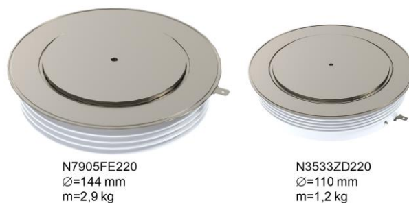
Figure 9: Comparison between the N7905FE220 (resettable) and N3533ZD200 (single use) Components
