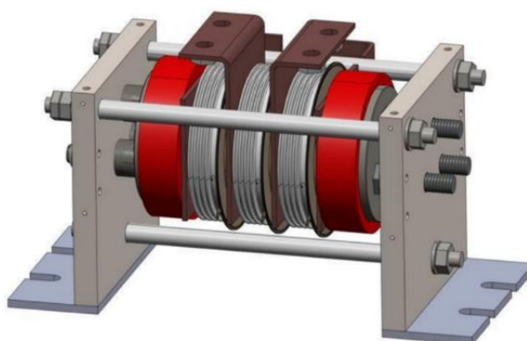
Figure 7: Thyristor-based, 3-phase Crowbar in \Delta -connection
