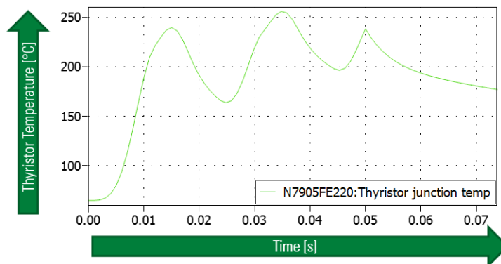
Figure 6: Estimated junction temperature development, N7905FE220
