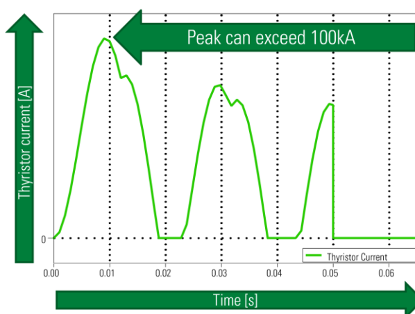
Figure 5: Short Circuit Current Simulation for a High-power Medium-voltage Transformer
