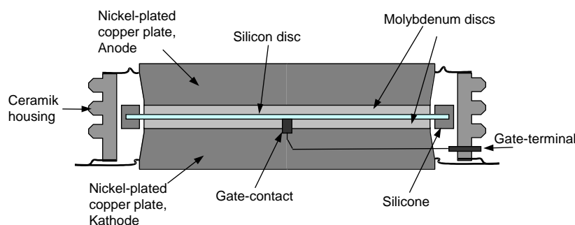
Figure 4: Cross-section of High-power Thyristor Disc-device
