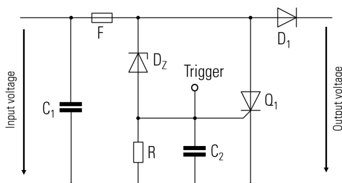
Figure 2: Low-power, DC-crowbar
