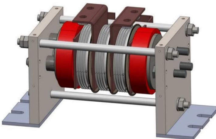
Figure 1: Thyristor-based, 3-phase Crowbar in \Delta -connection
