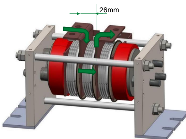
Figure 13: Closest proximity for Parallel Conductors in the Crowbar Stack
