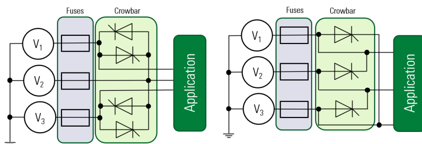
Figure 3: Crowbar Schematics in 3-phased Applications (Y-connected setup to the left and Δ-connected setup to the right)
