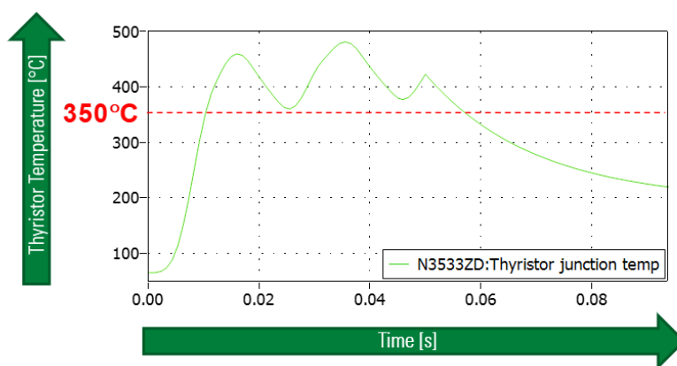
Figure 8: Estimated Junction Temperature Development, N73533ZD
