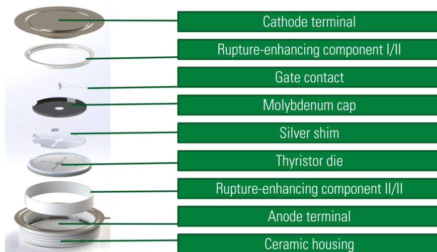
Figure 10: Components of the Rupture-enhanced Package Technology
