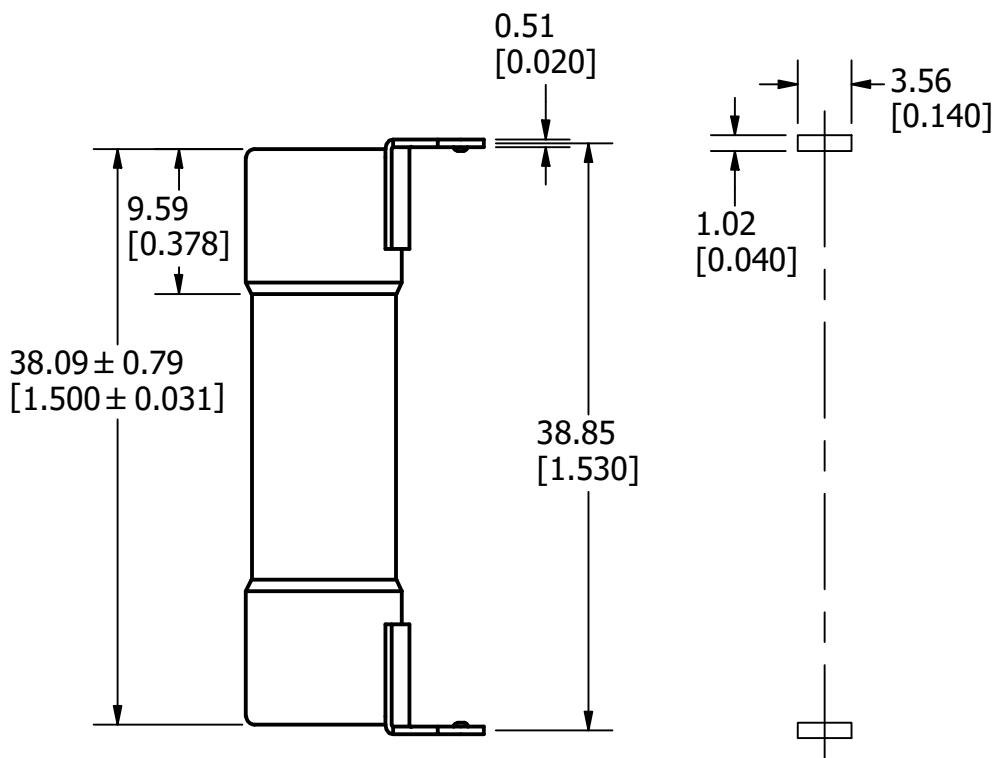
MOUNTING HOLE DETAIL
