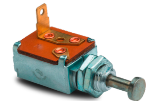
91812 12V 5A Normally Closed Self Grounded Door Switch
