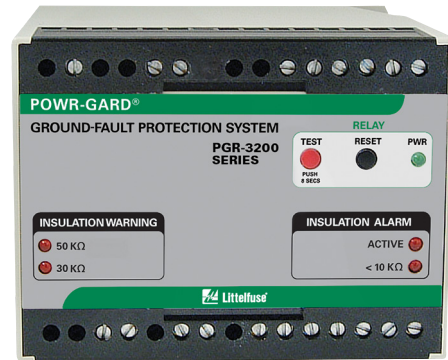
Figure 4. The Littelfuse POWR-GARD® PGR-3200 Insulation Monitor can be used with both ungrounded and grounded BESSs.
