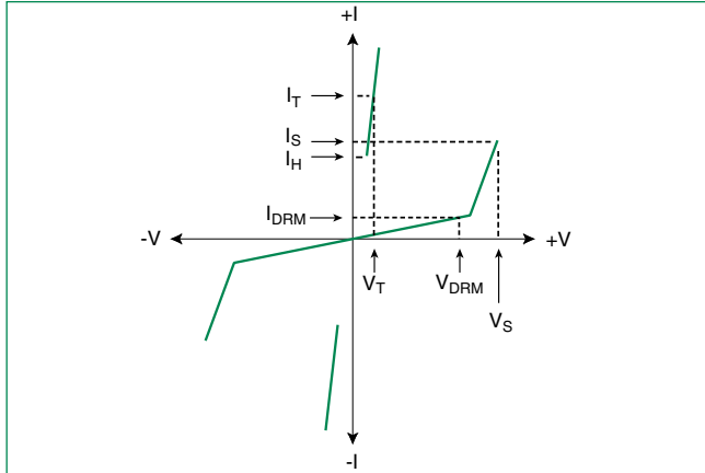
V-I Characteristics
