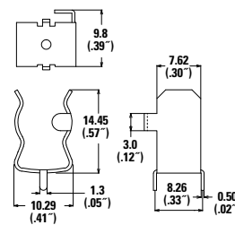
106 001 Device Dimensions
