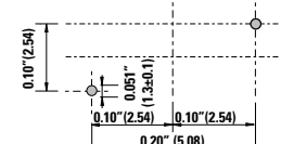
Circuit Board Mounting Detail
