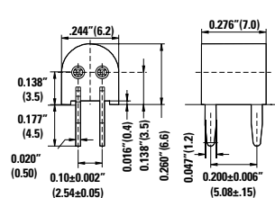
Circuit Board Mounting Detail
