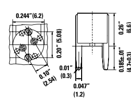
Circuit Board Mounting Detail
