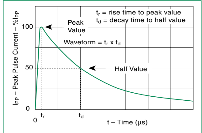
t_r \times t_d Pulse Waveform
