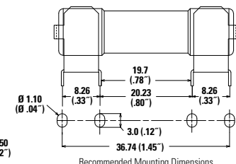
106 001 Device Dimensions
