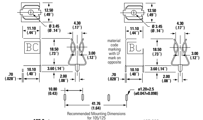
105 003 Device Dimensions
