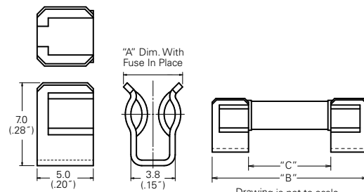
111 505 Device Dimensions
